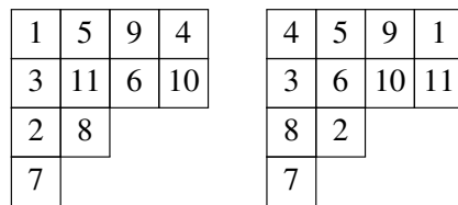
Figure 2: Two ( row- )equivalent Young tableaux.
